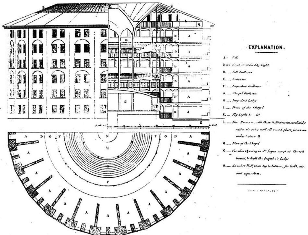
A General Idea of a PENITENTIARY PANOPTICON in an Improved, but as yet (Jan 23 d 1791), Unfinished State. See Postscript References to Plan, Elevation, & Section (being Plate referred to as A. 2).
